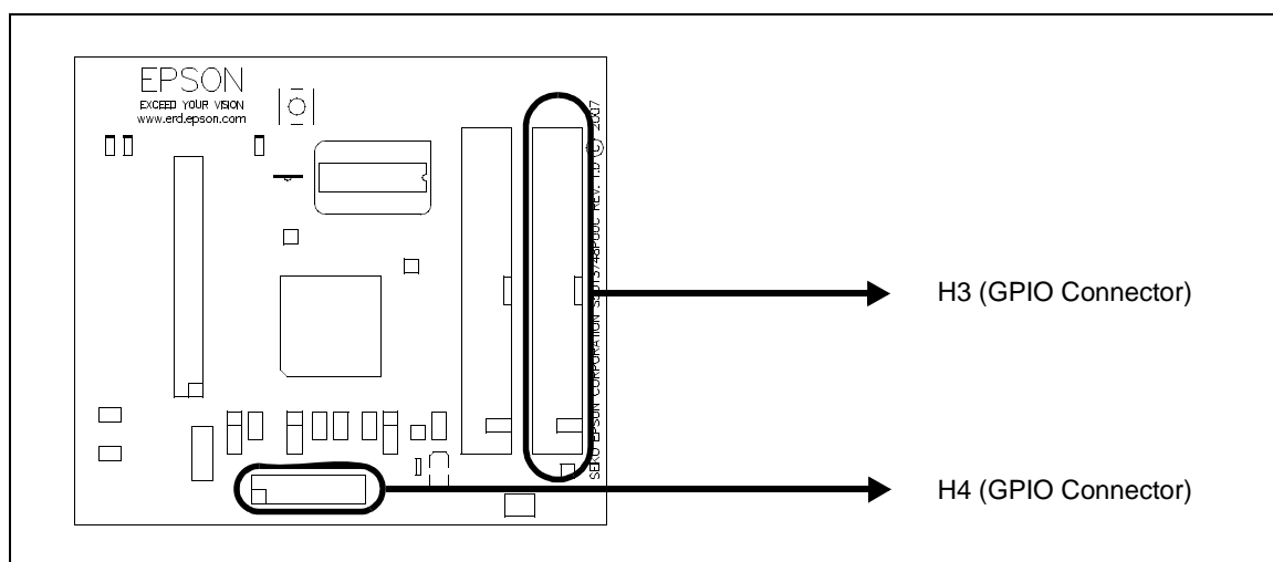
Figure 4-5: GPIO Connector Location (H3, H4)
