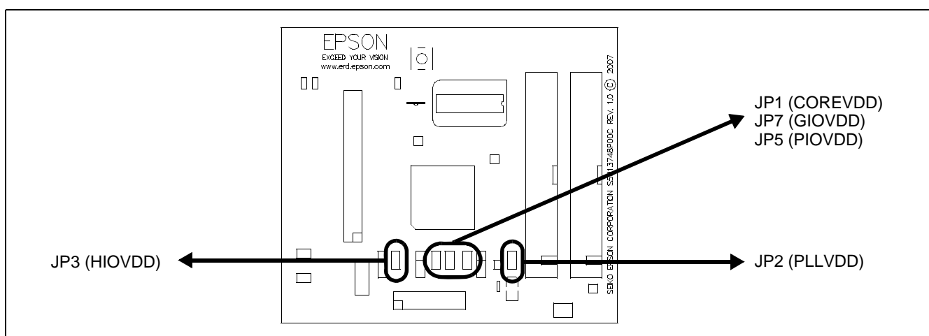
Figure 3-2: Configuration Jumper Locations (JP1, JP2, JP3, JP5, JP7)
