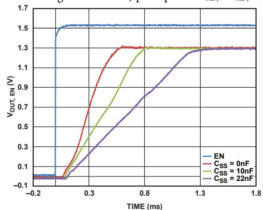
Figure 25. Fixed V_{\text{OUT}} Ramp-Up with External Soft Start Capacitor ( V_{\text{OUT, EN}} ) vs. Time
