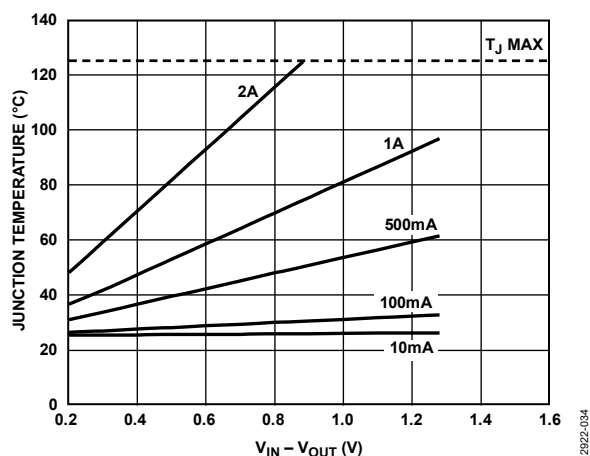
Figure 34. 6400 mm² of PCB Copper, T_A = 25^\circ\text{C}
