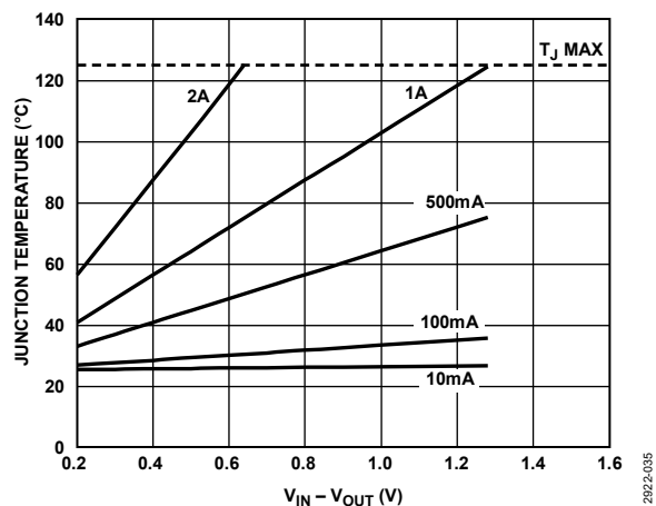
Figure 35. 500 mm² of PCB Copper, T_A = 25^\circ\text{C}
