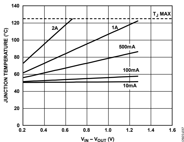
Figure 37. 6400 mm² of PCB Copper, T_A = 50^\circ\text{C}
