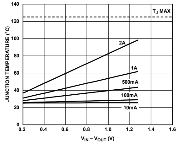
Figure 42. 1000 mm² of PCB Copper, T_B = 25^\circ\text{C}
