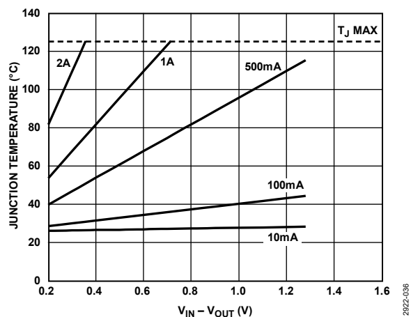
Figure 36. 25 mm² of PCB Copper, T_A = 25^\circ\text{C}
