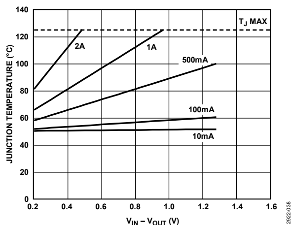
Figure 38. 500 mm² of PCB Copper, T_A = 50^\circ\text{C}
