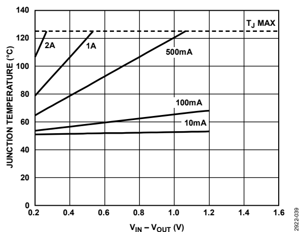
Figure 39. 25 mm² of PCB Copper, T_A = 50^\circ\text{C}
