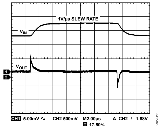
Figure 16. Line Transient Response, Load Current = 2 A, V_{IN} = 1.5\text{ V} to 1.98\text{ V} Step, V_{OUT} = 1.3\text{ V}
