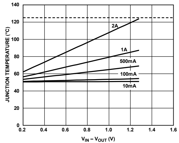
Figure 43. 1000 mm² of PCB Copper, T_B = 50^\circ\text{C}
