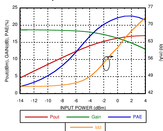
Power Compression @ 1700 MHz [2]
