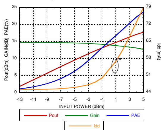
Power Compression @ 2100 MHz [2]
