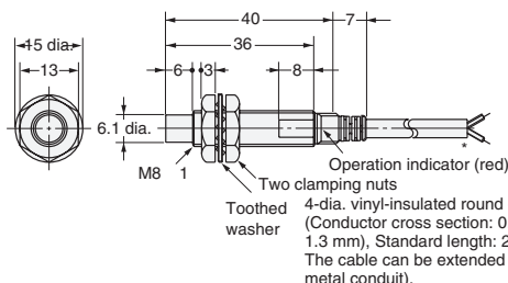
Diagram 10 E2E-X8MD□ Pre-wired e-CON Connector Models E2E-X5ME□/F□
