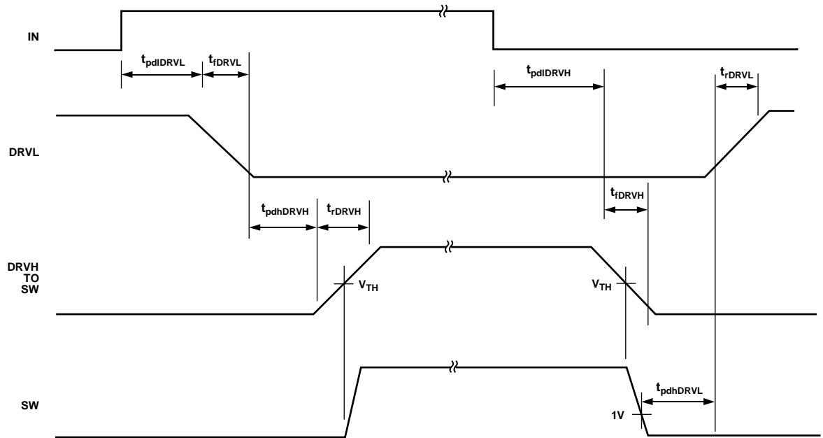
Figure 3. Timing Diagram
