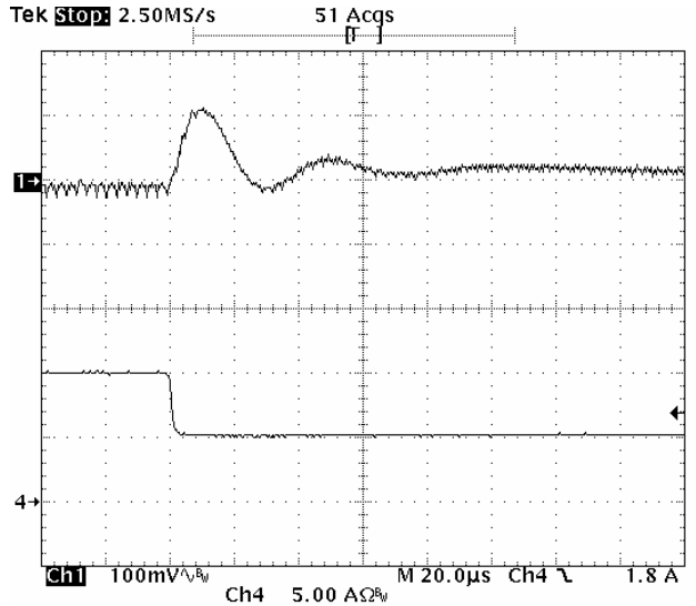
Fig-2.5V-7: Output voltage response for V_{out}=2.5V to positive load current step-change from 10A to 5A with slew rate of -5A/\mu s at V_{in}=5.0V . C_o=47\mu F \times 4 ceramic + 1\mu F ceramic. Top trace: output voltage (100mV/div.) Bottom trace: load current (5A/div.) Time scale: 20µs/div.
