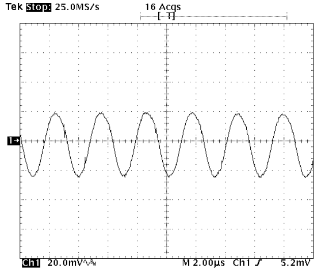
Fig-2.5V-5: Output voltage ripple (20mV/div.) for V_{out}=2.5V at full rated load current into a resistive load with external capacitance 47\mu F \times 4 ceramic + 1\mu F ceramic at V_{in}=5.0V . Time scale: 2µs/div
