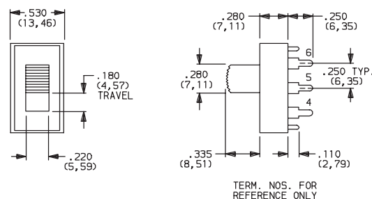
S202031MS02Q DPDT
