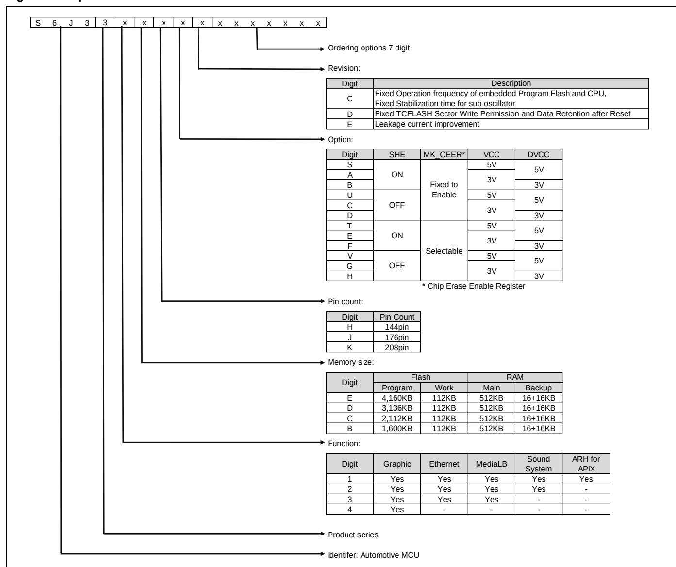
Figure 2-1: Option and Part Number for S6J3310/20/30/40 Series
