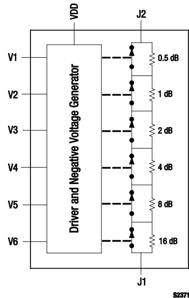
Figure 1. SKY12353-470LF Block Diagram
