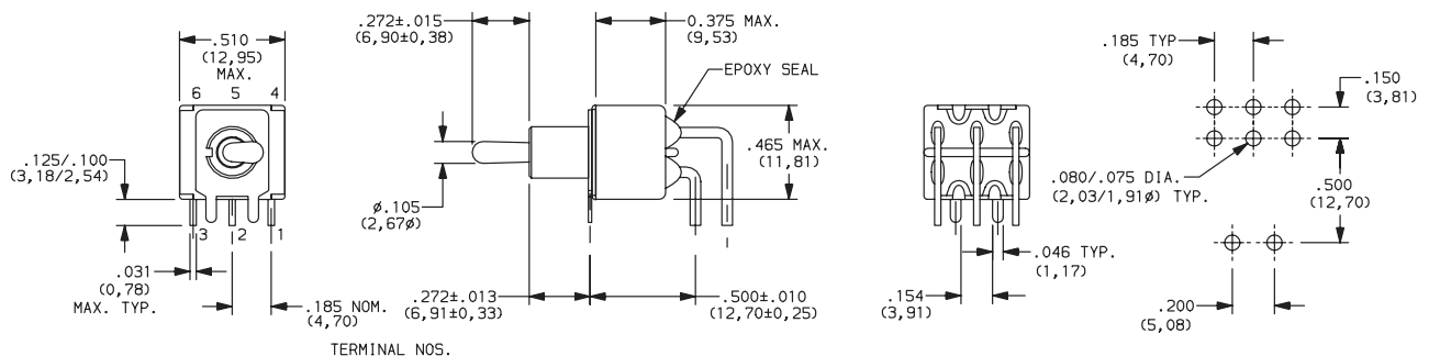
DPDT
