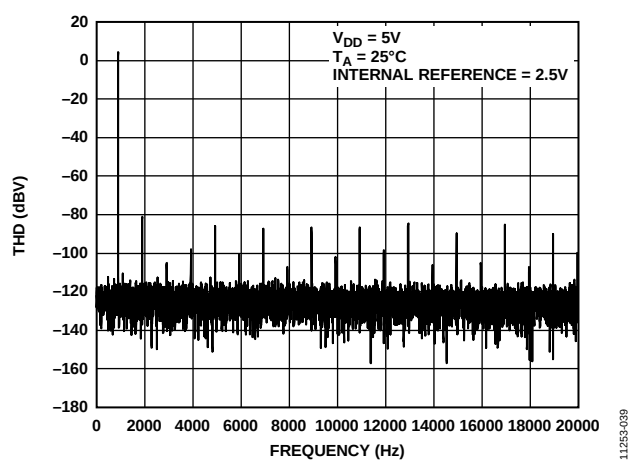
Figure 37. Total Harmonic Distortion at 1 kHz
