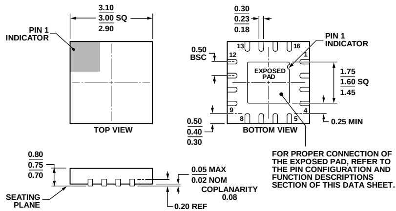
Figure 53. 16-Lead Lead Frame Chip Scale Package [LFCSP_WQ] 3 mm × 3 mm Body, Very Very Thin Quad (CP-16-22)
