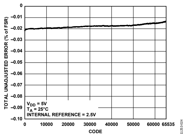
Figure 22. Total Unadjusted Error vs. Code
