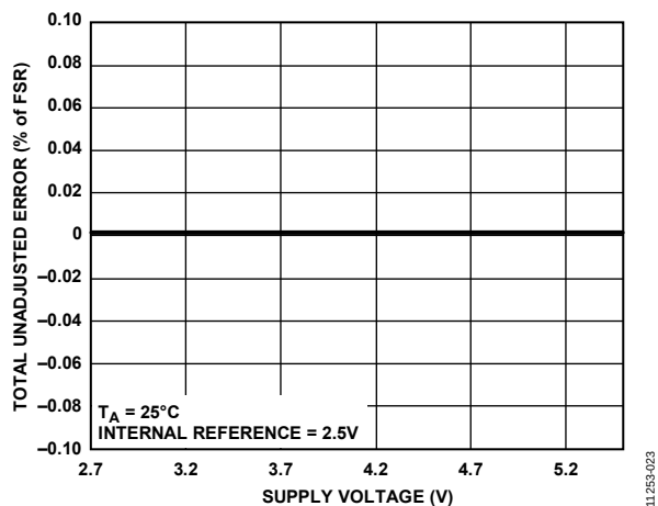
Figure 21. Total Unadjusted Error vs. Supply Voltage, Gain = 1
