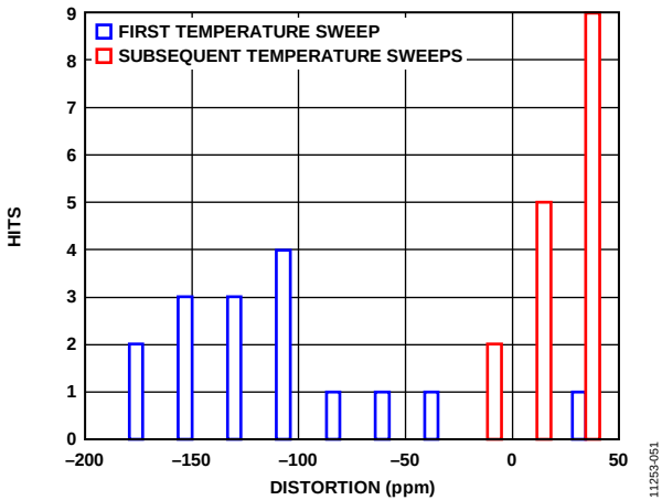
Figure 49. Thermal Hysteresis
