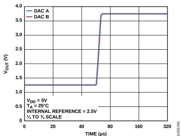
Figure 29. Settling Time
