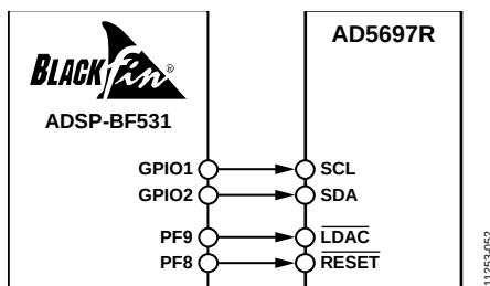
Figure 50. ADSP-BF531 Interface to the AD5697R
