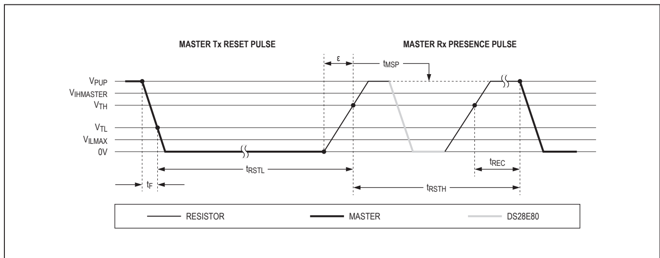
Figure 9. Reset/Presence pulse
