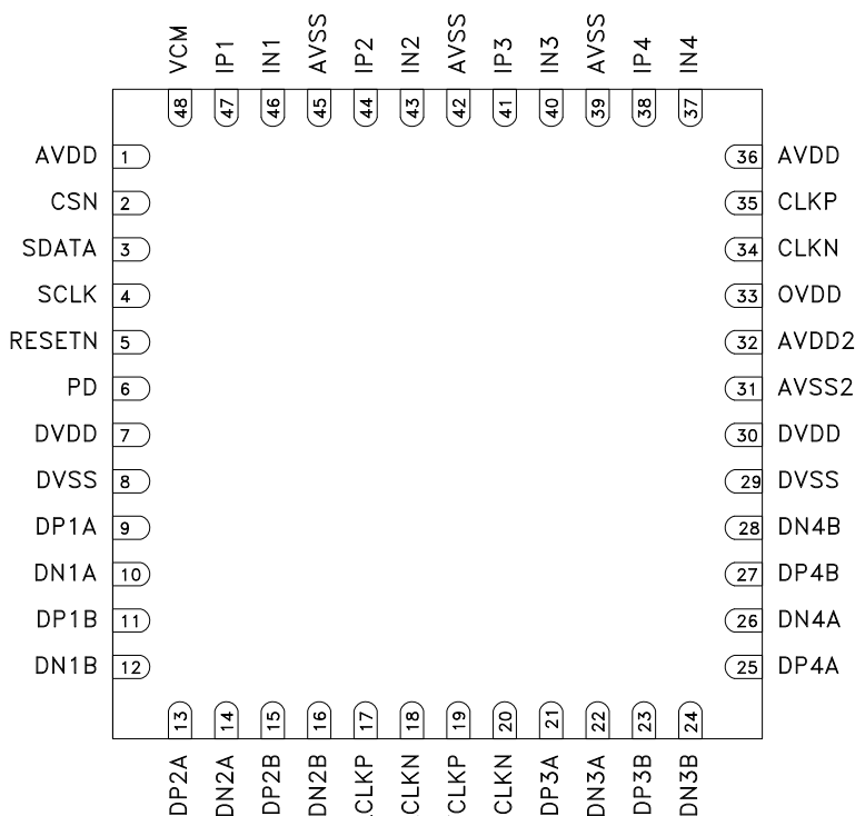
Figure 2: Package diagram
