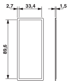
Dimensional drawing
