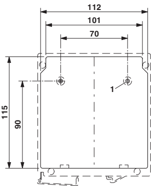
Dimensional drawing
