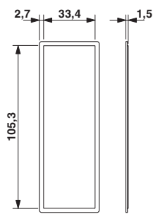
Dimensional drawing
