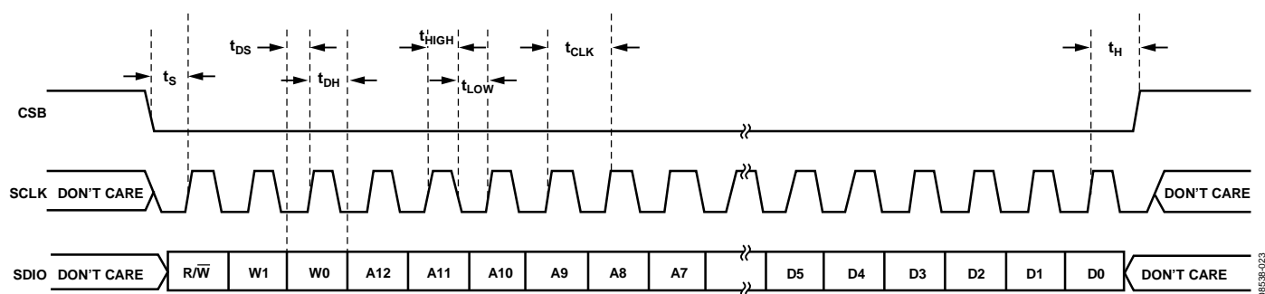
Figure 59. Serial Port Interface Timing Diagram
