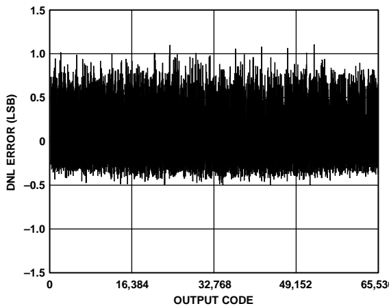
Figure 14. DNL Error with f_{IN} = 9.7 MHz
