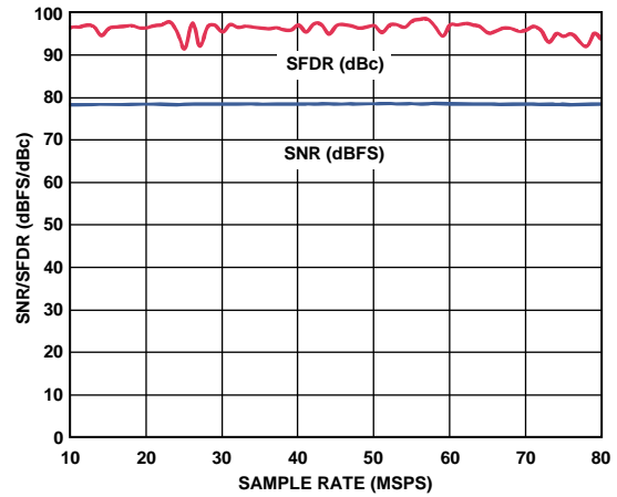
Figure 13. AD9269-80 SNR/SFDR vs. Sample Rate with f_{IN} = 9.7 MHz
