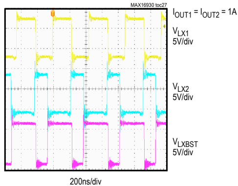
LX WAVEFORMS
