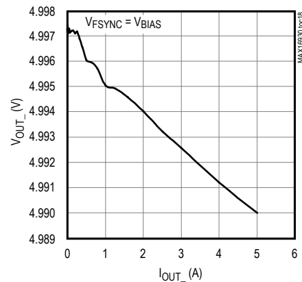
BUCK 1 LOAD REGULATION
