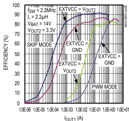
BUCK 2 EFFICIENCY
