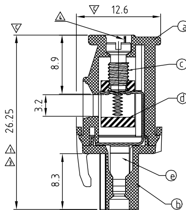
SECTION P-P
