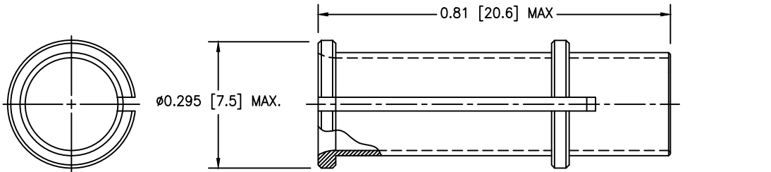
-01: PASS-THROUGH
