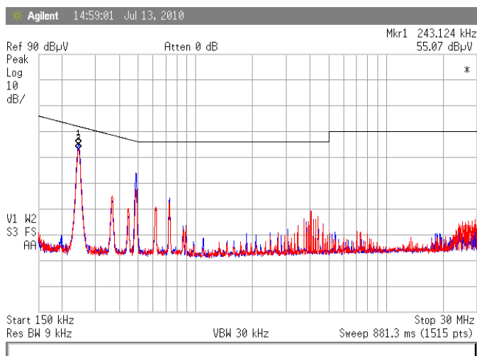
Figure 6 – Ericsson PKM4304B PI using base-plate “Y” capacitors with a 360W load, CX1 = 47μF (see Figure 2).
