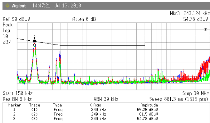
Figure 7 – CM Peak Measurements with a 10μF and 47μF CX1 capacitor.
