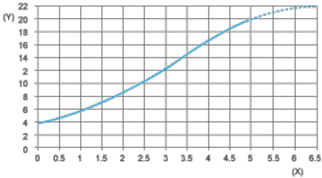
(Y) Is (mA) (X) Sensors - object distance (mm)
