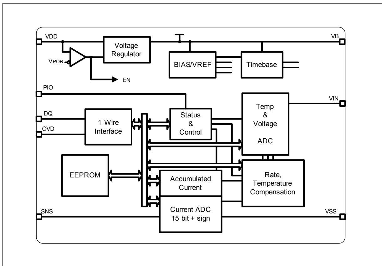
Figure 1. Block Diagram
