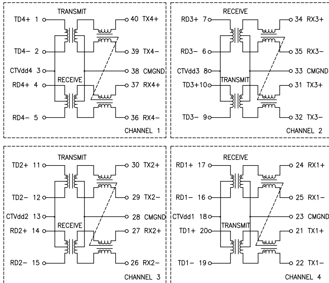
SCHEMATIC
