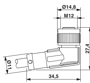
M12 x 1 socket, angled
