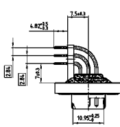
View without clip
