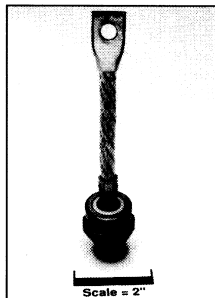
IN3260, R - IN3276, R General Purpose Rectifier 160 Amperes Average, 1600 Volts
