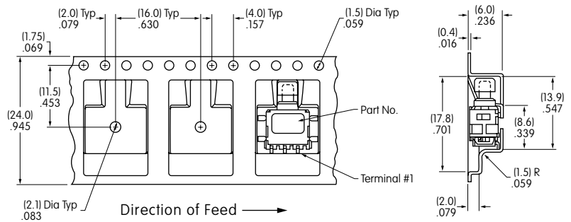
Tape Dimensions
