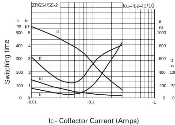
Switching Speeds
