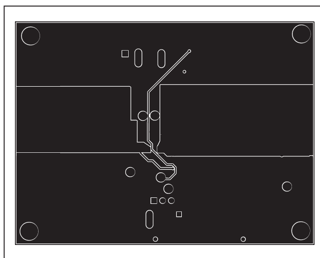
Figure 4. MAX15090 EV Kit PCB Layout—Layer 2 (PWR/GND)
