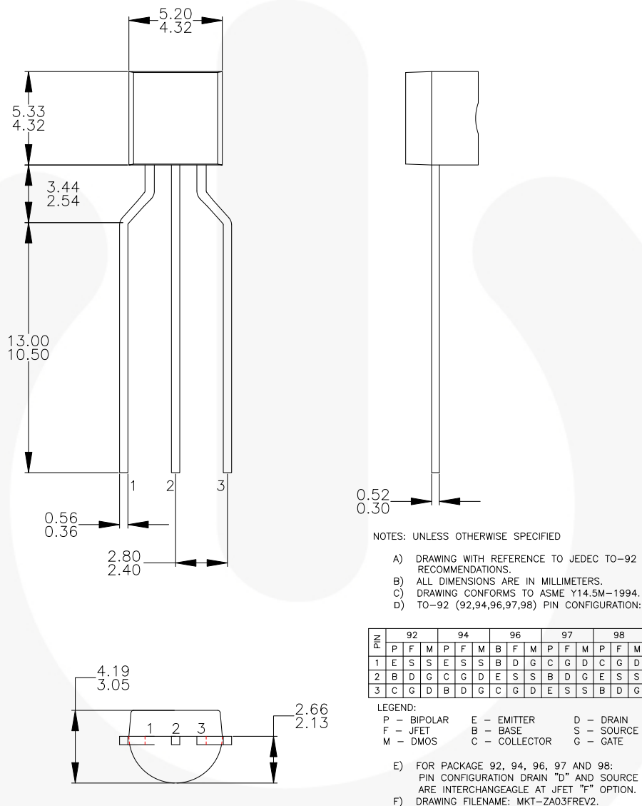
Figure 11. 3-LEAD, TO92, MOLDED, 0.200 IN-LINE SPACING LD FORM(J62Z OPTION) (ACTIVE)
