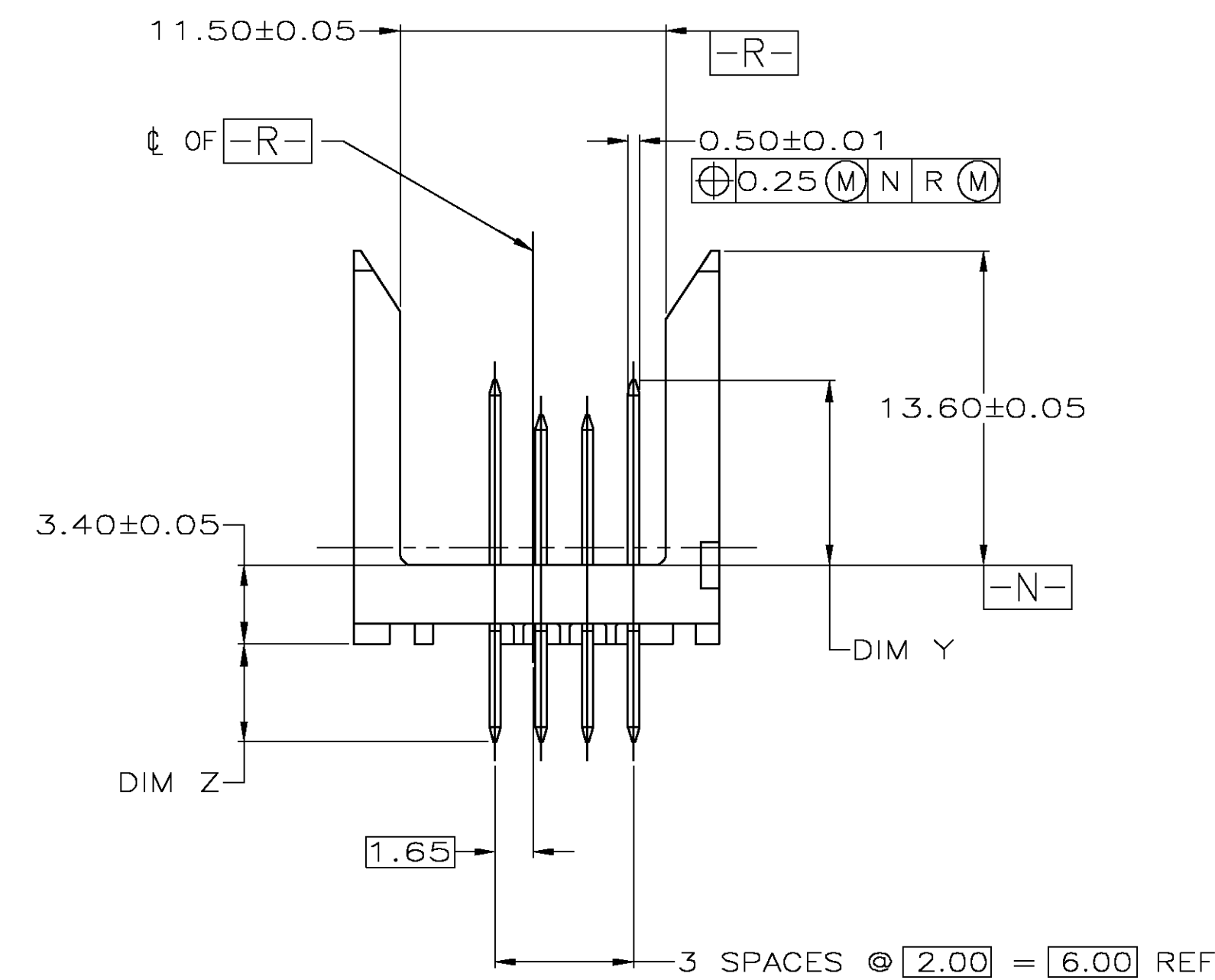
5536699-1 AS SHOWN
