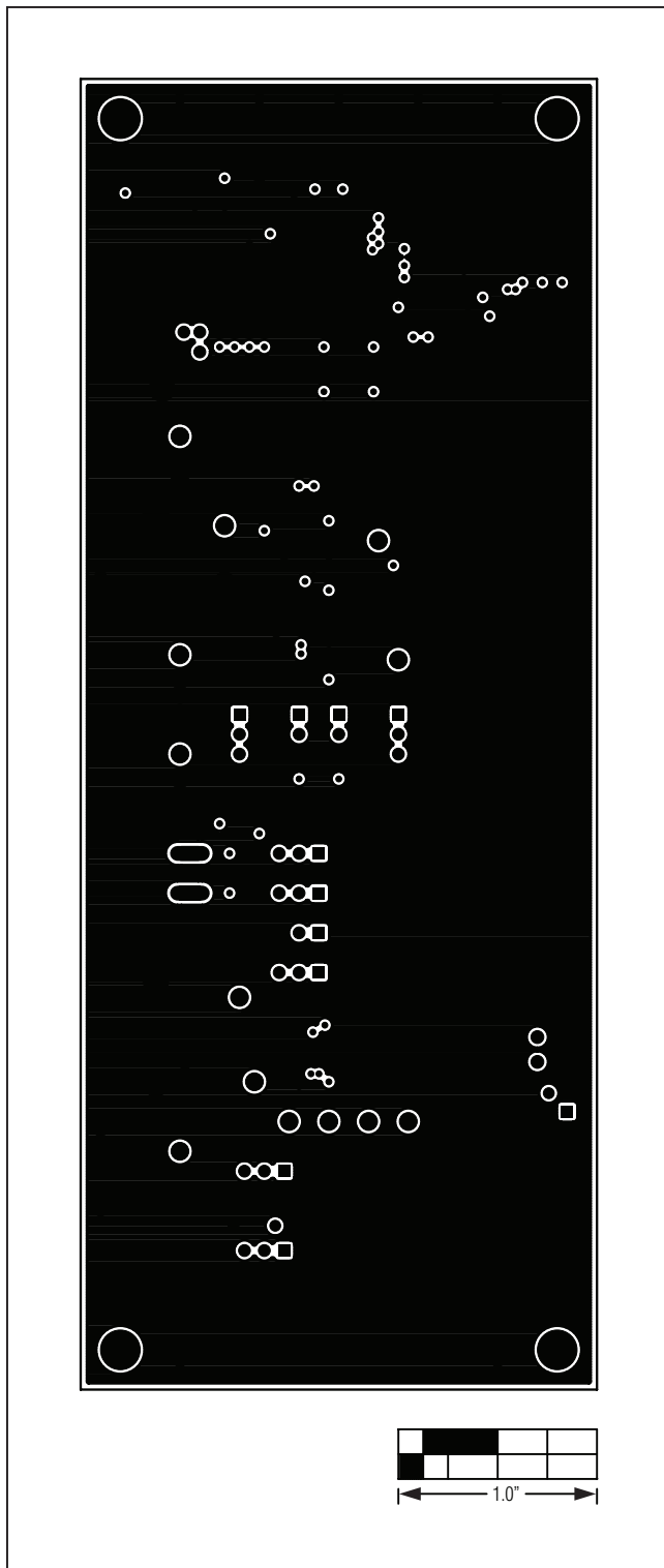
Figure 7. MAX14578 EV Kit PCB Layout—Layer 2
