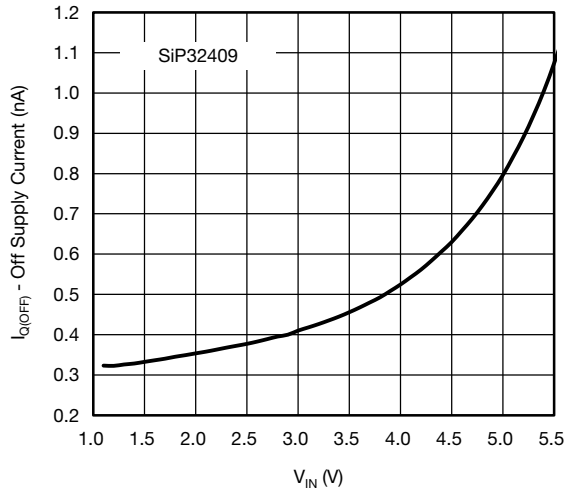
Figure 7 - Off Supply Current vs. Input Voltage
