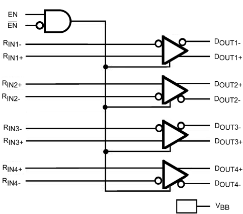
Functional Diagram
