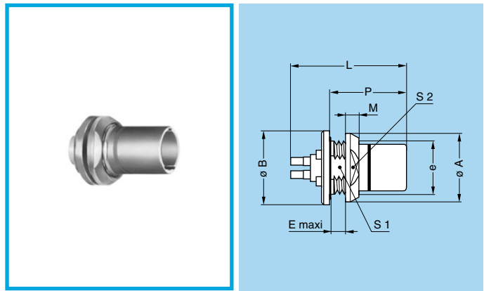
EH● Fixed socket, nut fixing, key (N) or keys (P and S), (back panel mounting)
