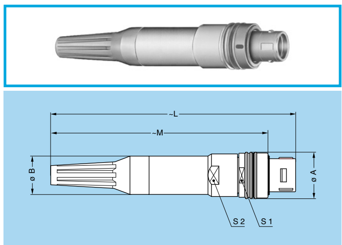
FG● Straight plug, key (N) or keys (P and S)
