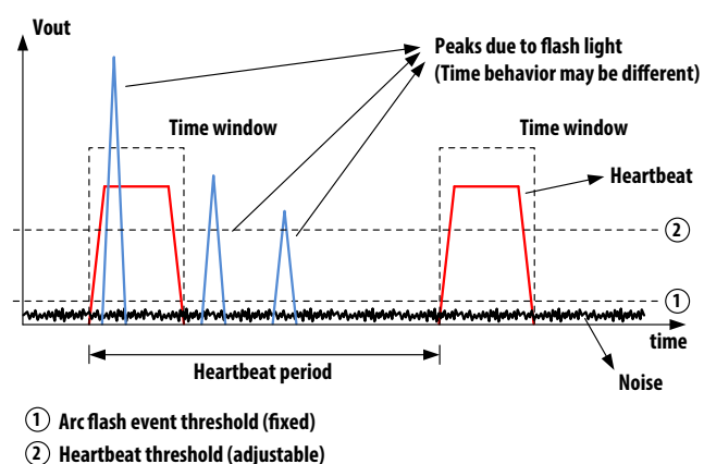
Figure 2. Schematic of the time window implemented in the Arduino microcontroller placed on AFBR-S10EB001Z
