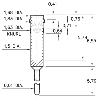
1305-0-15-XX-47-XX-04-0 Press-fit in 1,55 mounting hole
