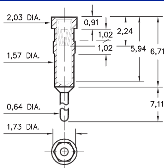
0335-0-15-XX-47-XX-04-0 Hex press-fit in .1,63 plated thru hole
