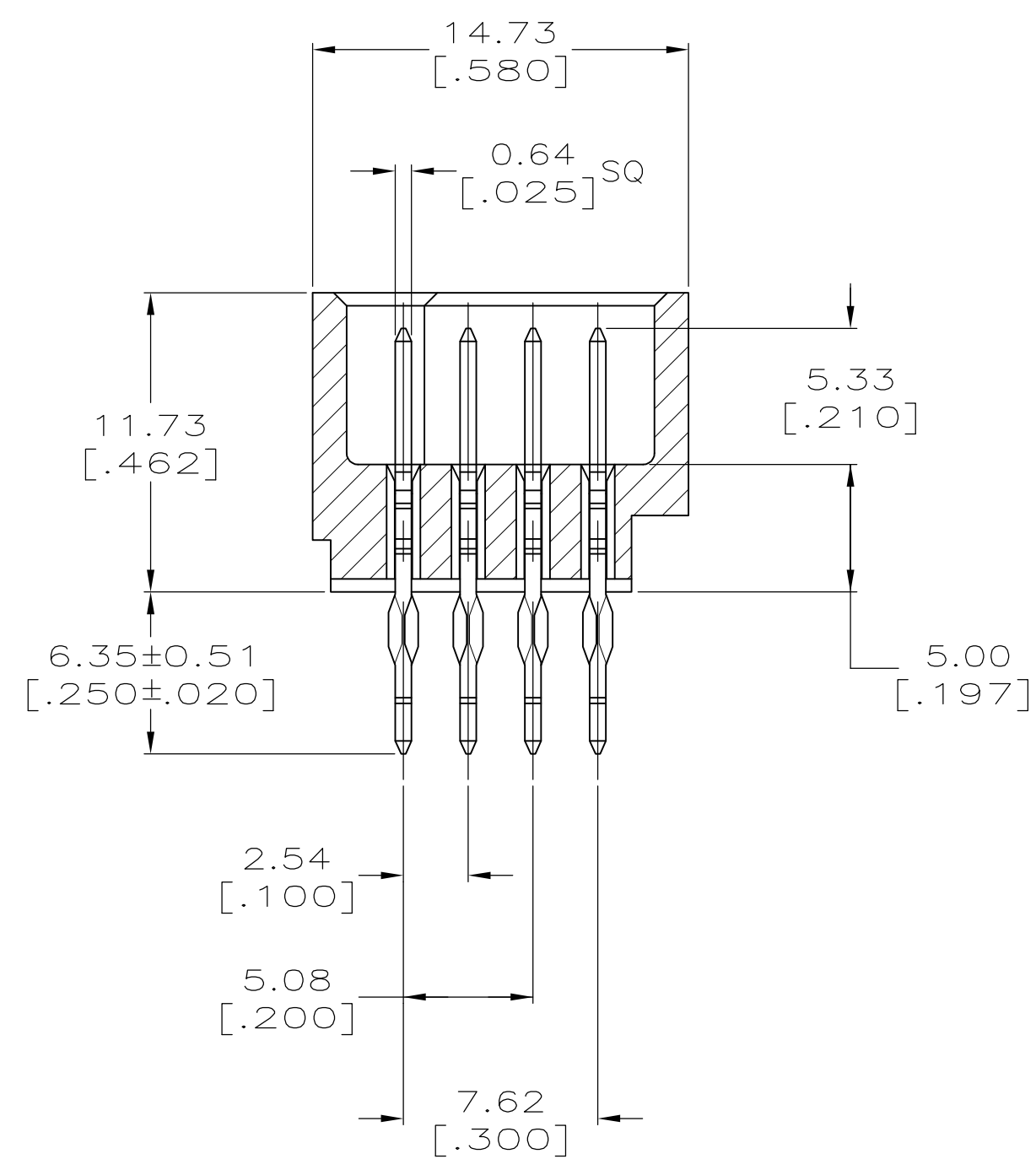
SECTION T-T
