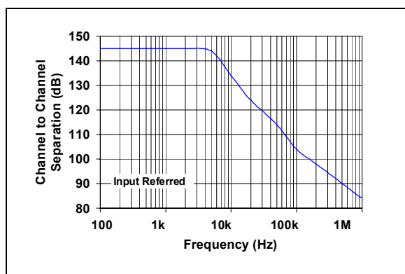
FIGURE 2-21: Channel-to-Channel Separation vs. Frequency (MCP6072/4 only).
