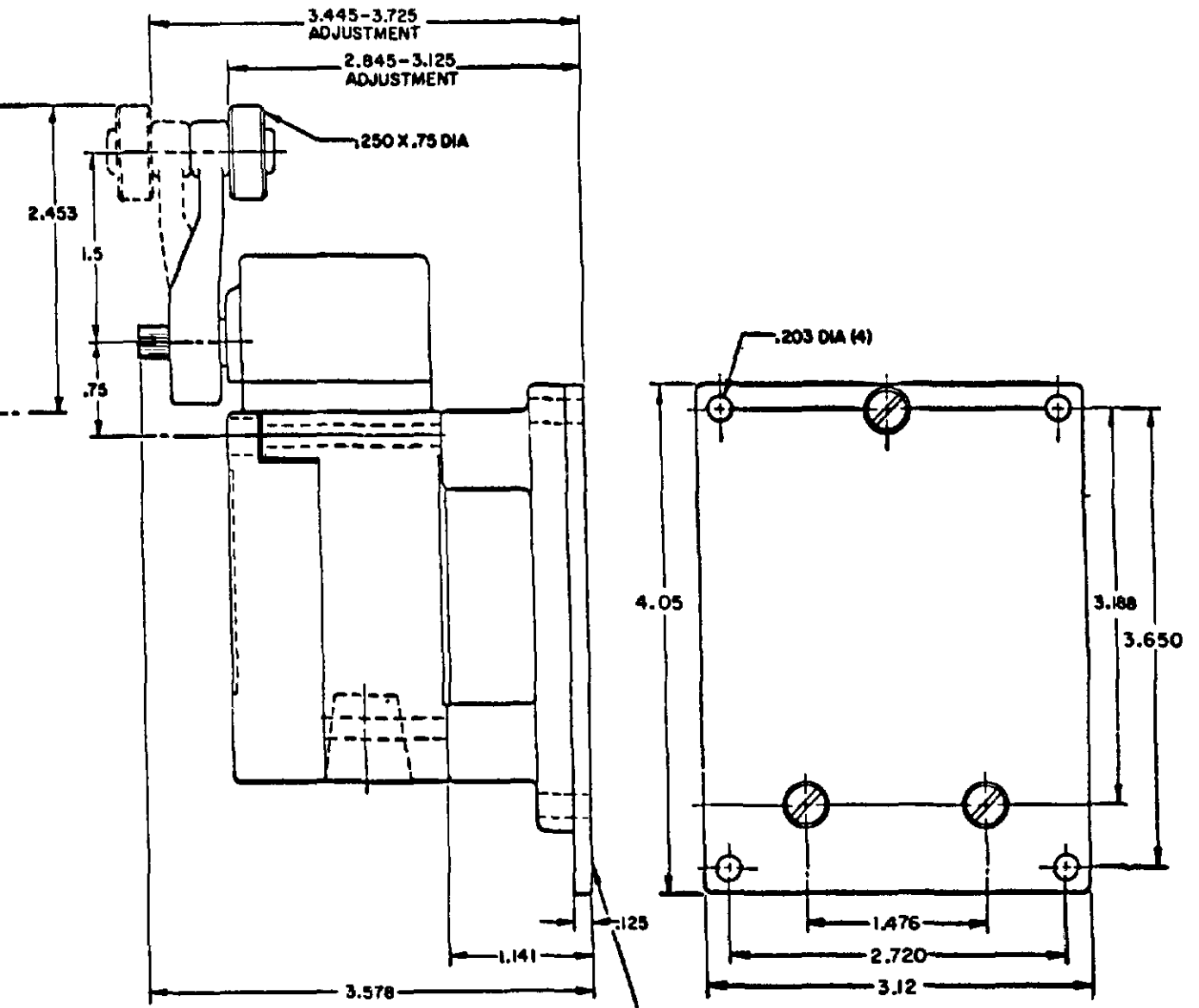
DOUBLE POLE (SIDE ROTARY) LSZ4004
