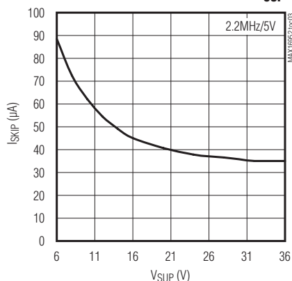
SKIP MODE SUPPLY CURRENT vs. V_{SUP}
