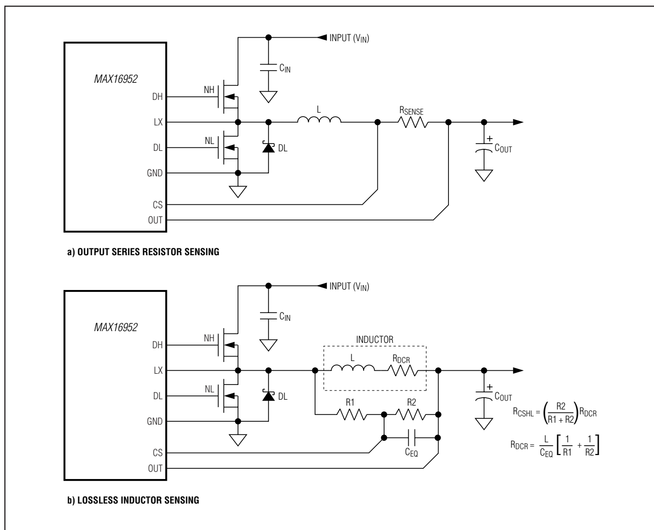
Figure 4. Current-Sense Configurations
