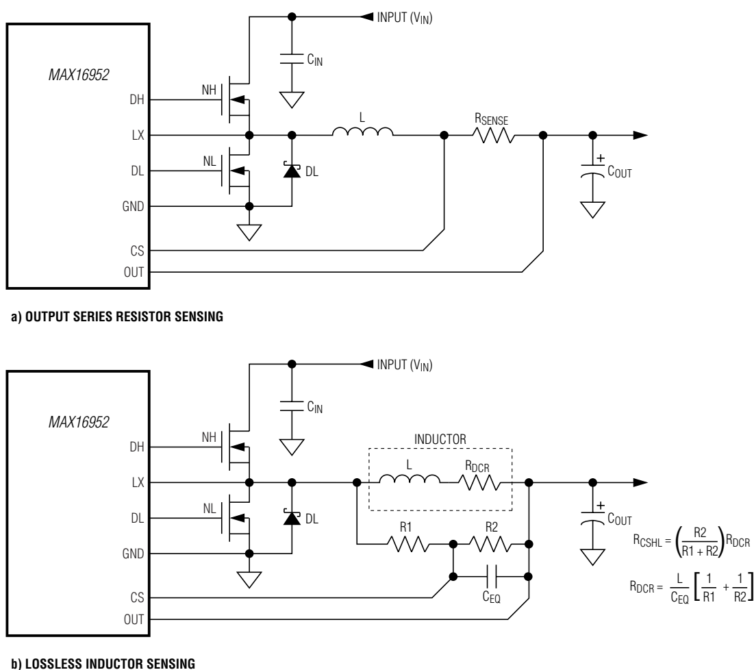
Figure 4. Current-Sense Configurations
