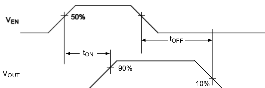
Figure 1a. MIC2546/47-1
