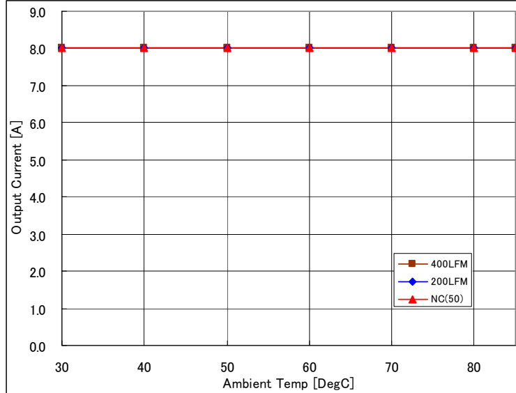
Fig 2.5V-1: Available load current vs. ambient temperature and airflow rates for Vout=2.5V with Vin=12V. Maximum component temperature \leq 120^{\circ}\text{C} .
