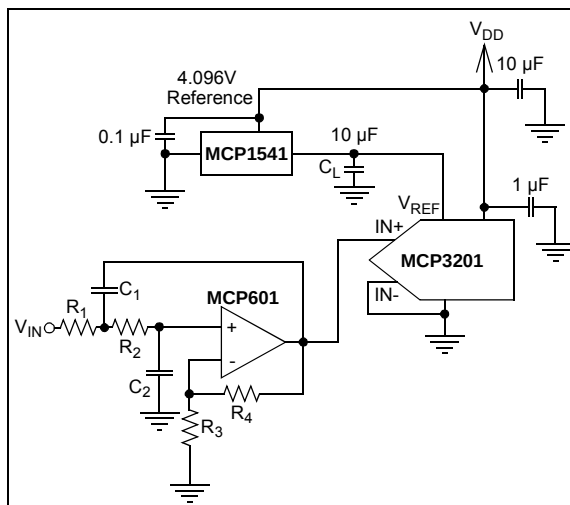
FIGURE 6-3: The MCP601 Operational Amplifier is used to implement a 2nd order anti-aliasing filter for the signal being converted by the MCP3201 device.
