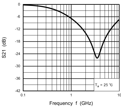
Fig. 9.5 S_{21} - f
