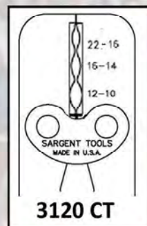
#3120 CT - Ratchet Conductor Crimp Tool
