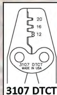
#3107 DTCT - Circular Contacts Ratchet Crimp Tool
