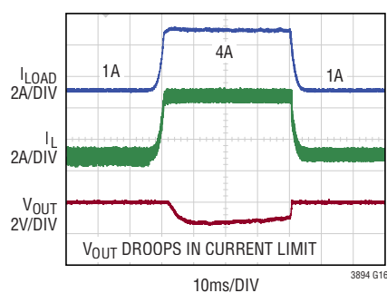
Overcurrent Protection
