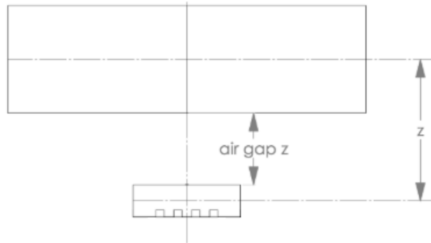
Figure 4: Magnet Air Gap Spacing
